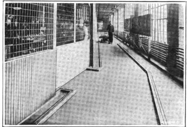
Fig. 6—In order for trucking to be done efficiently, it is of absolute importance that all aisles in the factory be kept open. Instead of a paint line down each side of the aisle, the Timken-Detroit Axle Co. uses 2 x 4 in. timbers protected with angle irons. These effectually prevent trucks running out of the aisles
